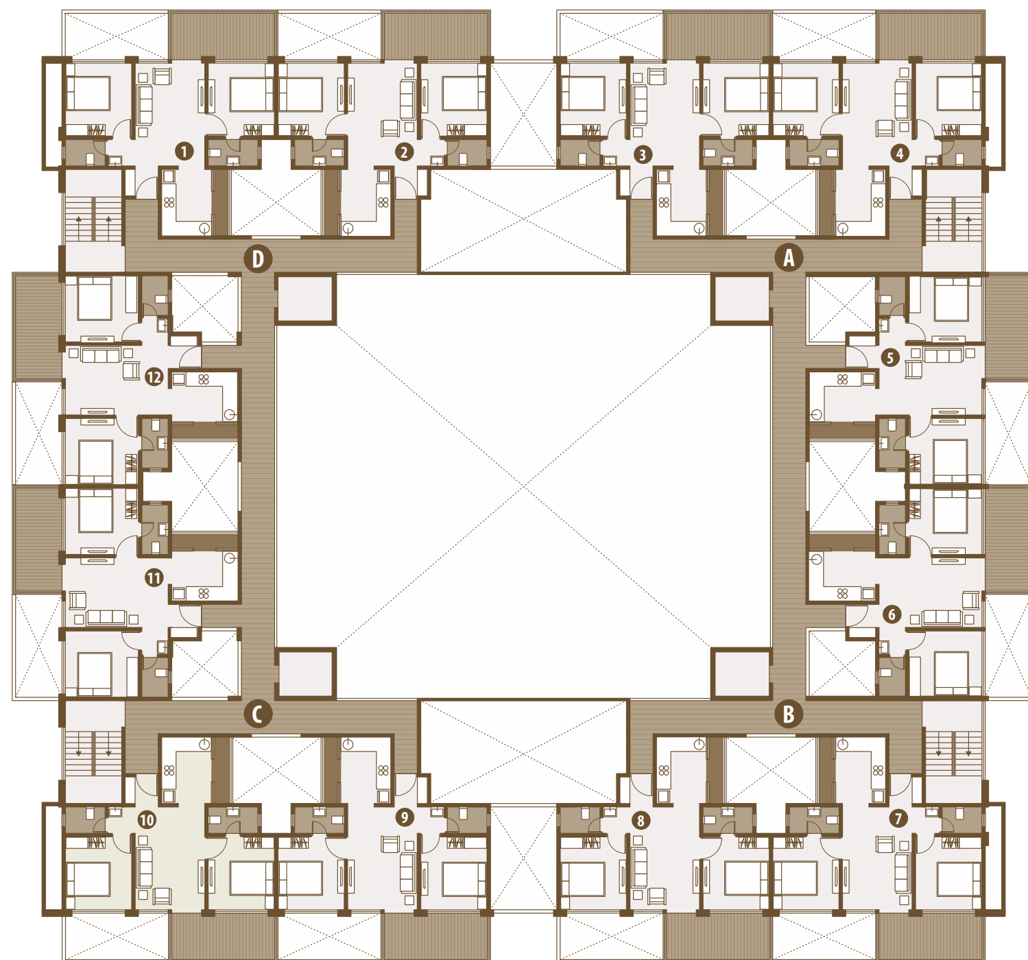
EVEN FLOOR PLAN Typ. 2nd,4th,6th,8th,10th & 12th
